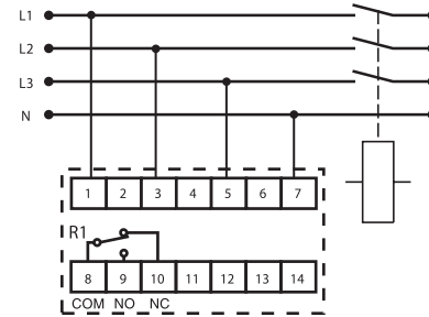
3-Phase System
