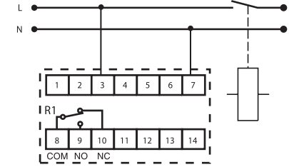
Single-Phase System
