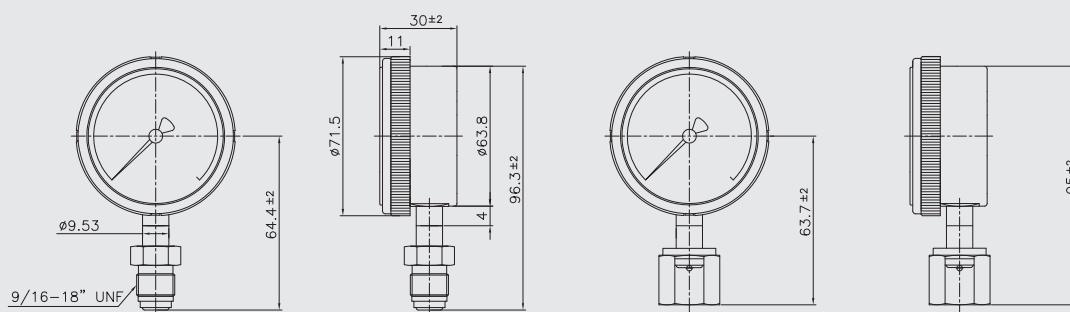
Swivel male
