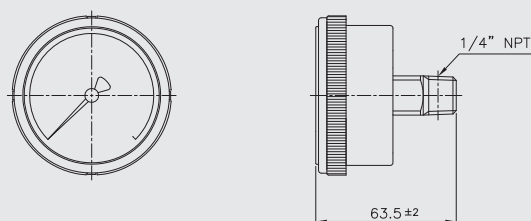
NPT male
