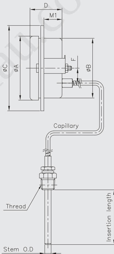
Dimensions (mm)
