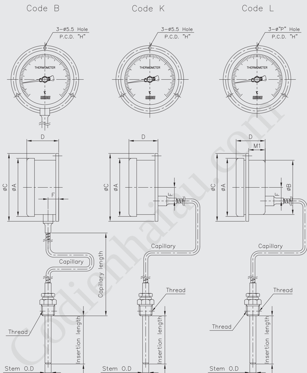
Dimensions (mm)
