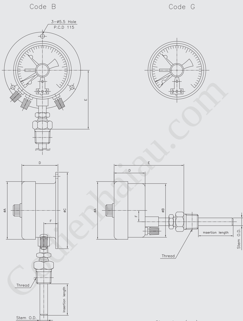
Dimensions (mm)
