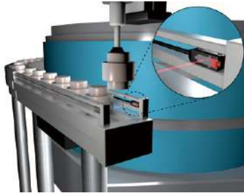
Detection of parts in parts feeder
